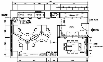
NPC INC. TAIWAN OFFICE FLOOR PLAN A1
